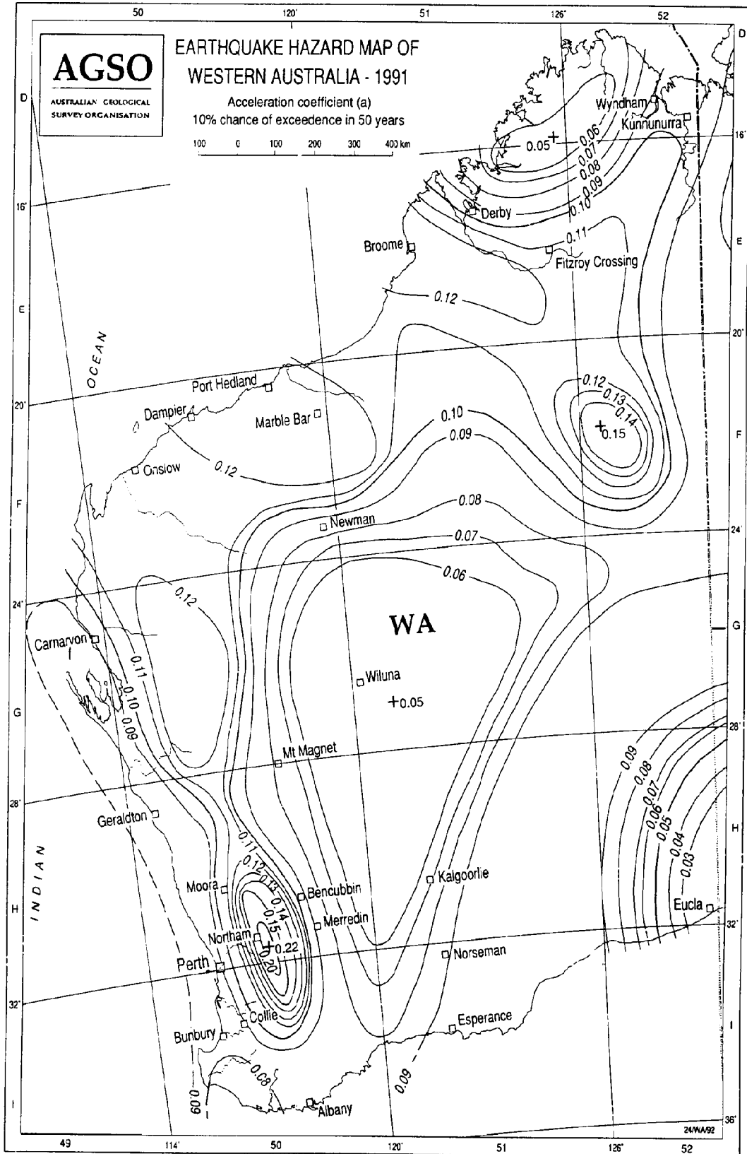
FIGURE 2.3(d) ACCELERATION COEFFICIENT MAP OF WESTERN AUSTRALIA
