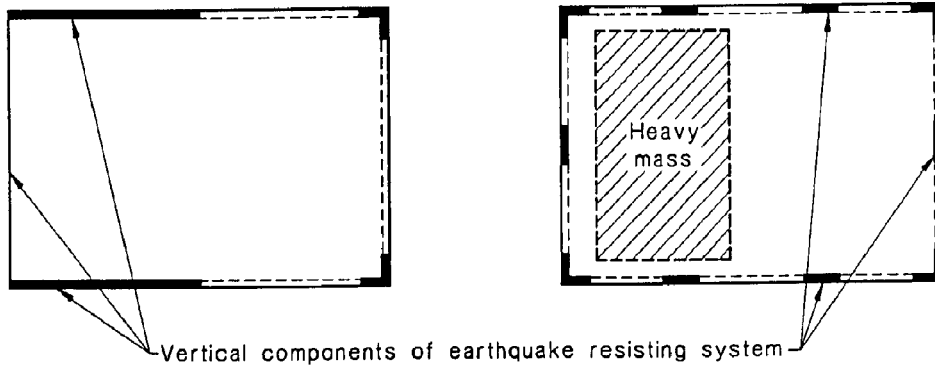
(b) Mass resistance eccentricity
