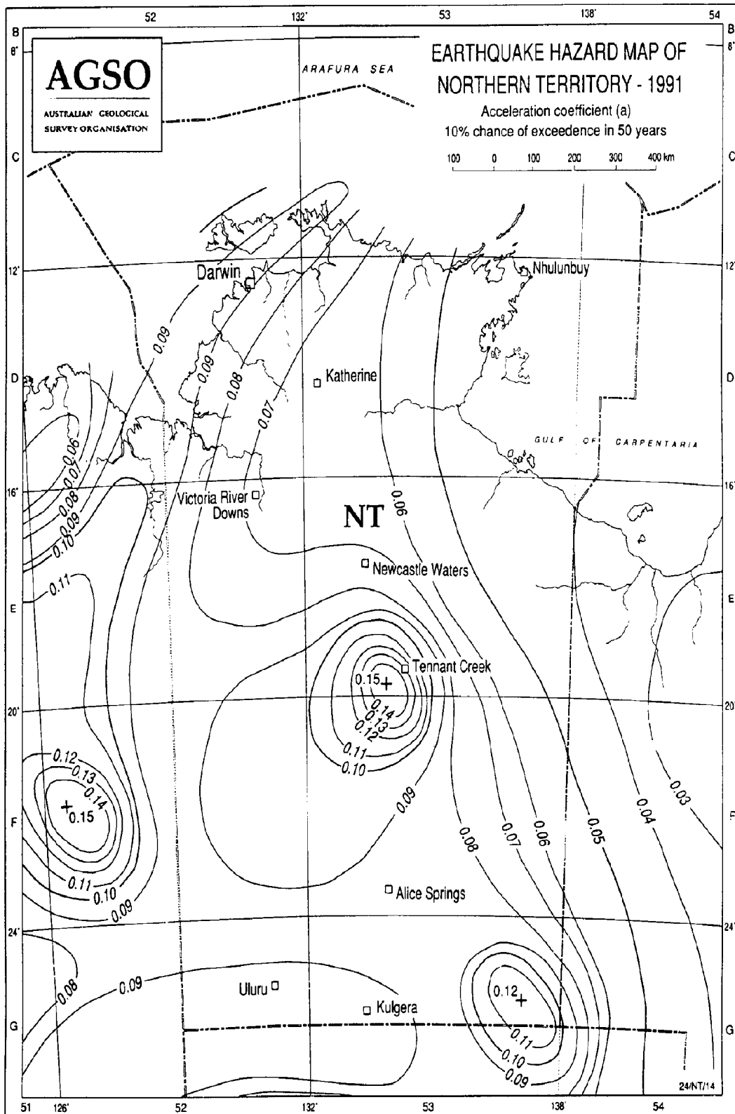
FIGURE 2.3(f) ACCELERATION COEFFICIENT MAP OF NORTHERN TERRITORY
